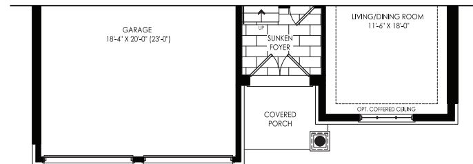
Elevation B Ground Floor
